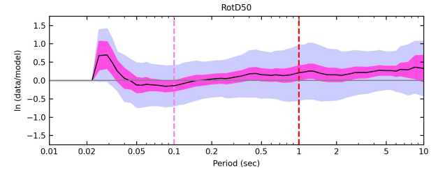
Goodness-of-fit plots
