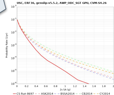
Hazard curves
