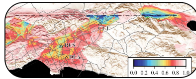
Wave Propagation (AWP-ODC)
