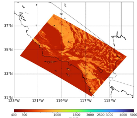
Velocity Model (UCVM)
